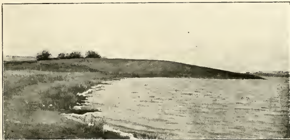
A. Sand dune advancing into Meyers Lake, near Pekin.
